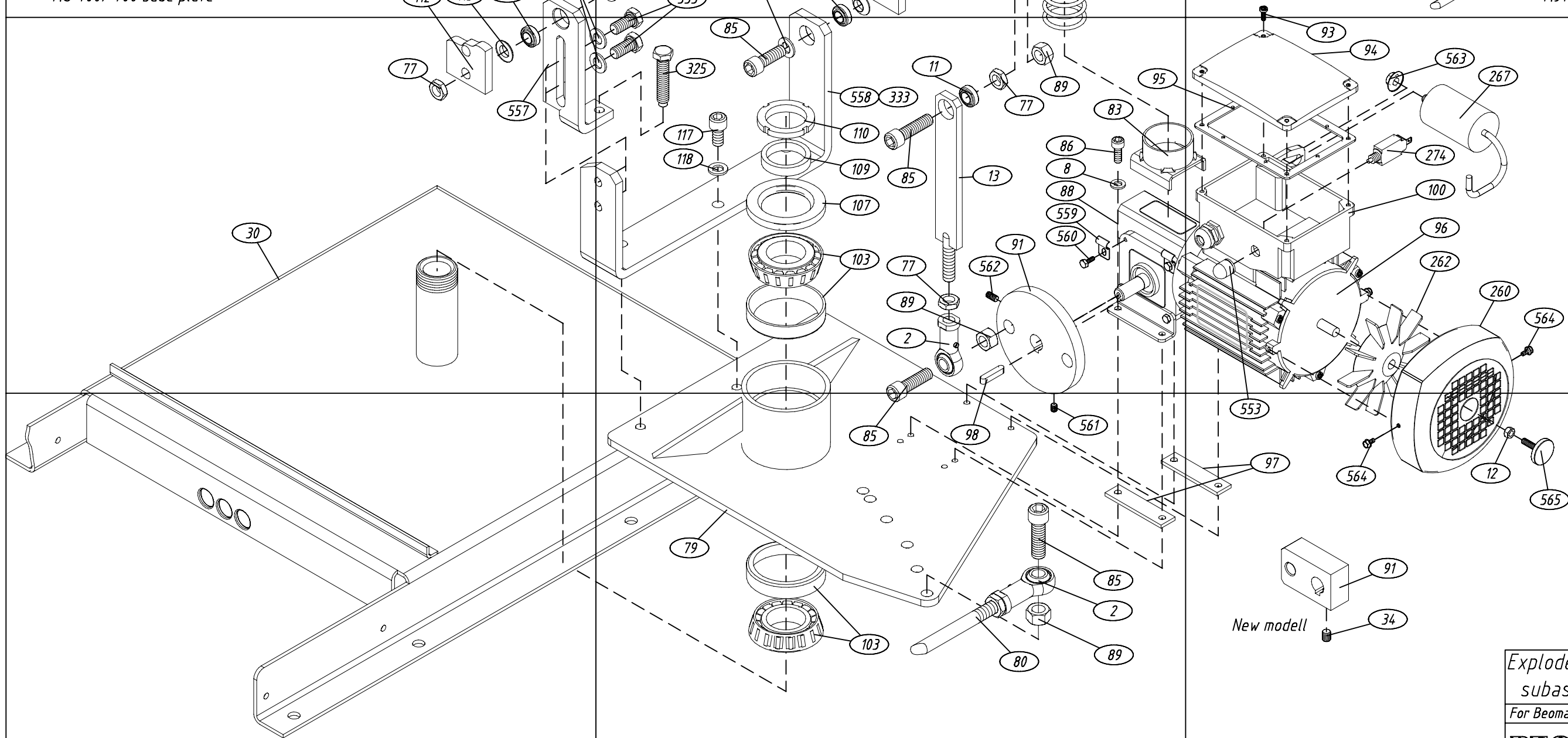
MJT 400 horizontal/ vertical drive plate
